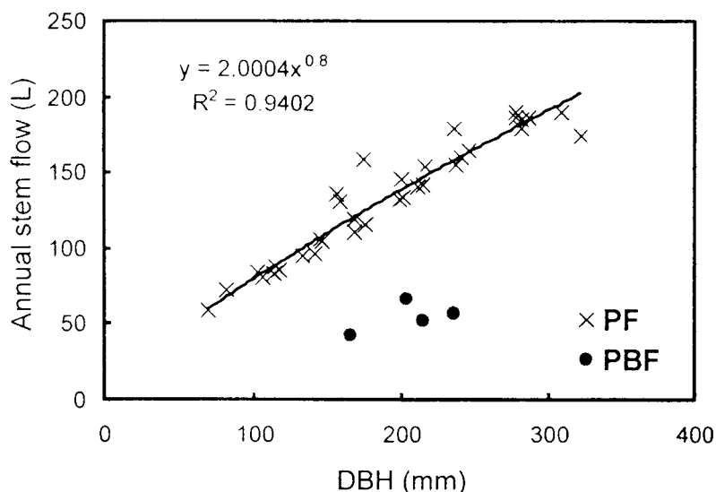
Fig. 11. The relationship between annual stem flow and diameter at breast height (DBH) for Masson pine ( Pinus massoniana ) trees growing in pine forest (PF) and mixed pine-broadleaf forest (PBF) communities.
