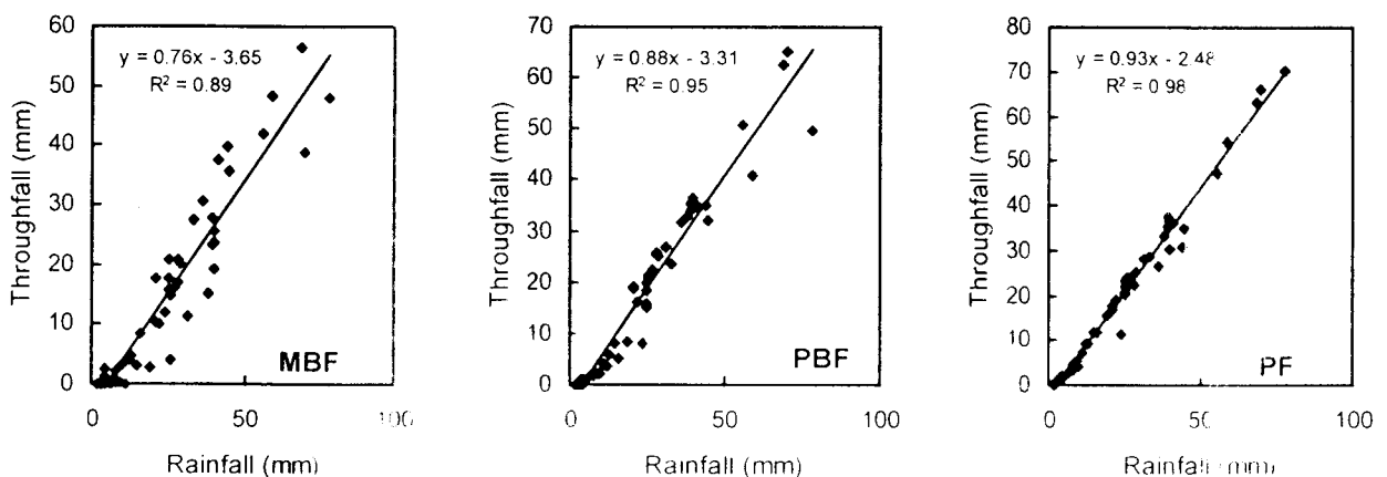
Fig. 10. Throughfall and rainfall in three successional vegetation communities at Dinghushan. PF, pine forest; PBF, mixed pine-broadleaf forest; MBF, monsoon overgreen broadleaf forest.
