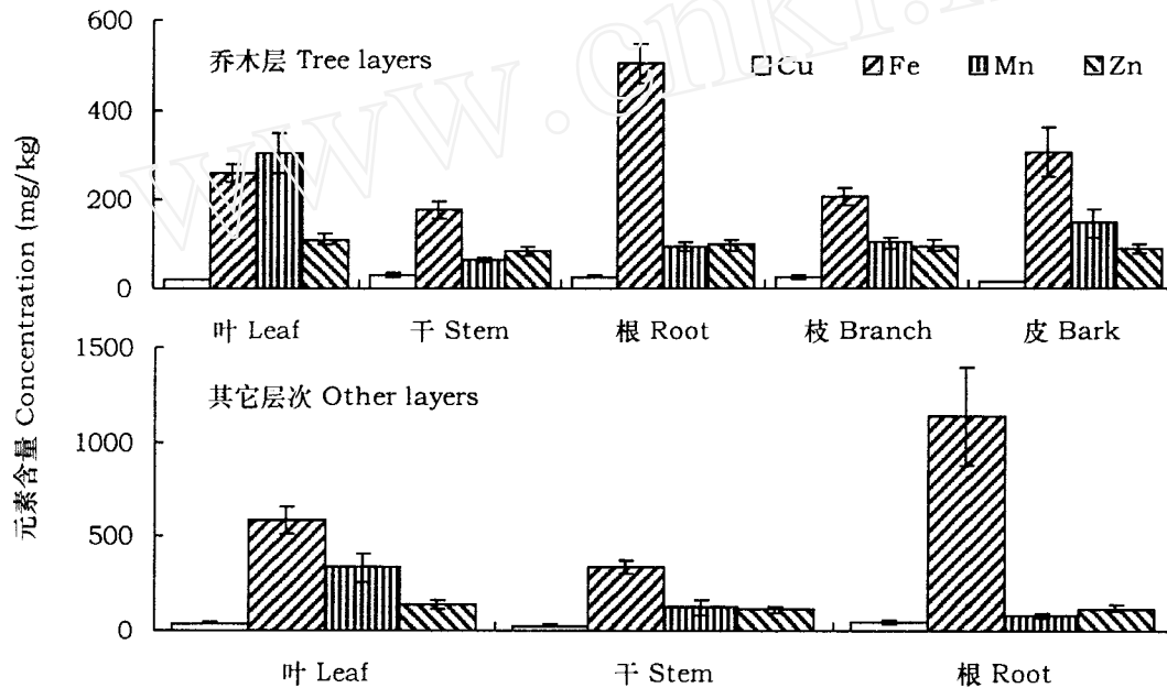
图 2 鼎湖山南亚热带常绿阔叶林植物各微量元素含量 Fig. 2 Minor nutrient element concentrations of plants in a lower subtropical evergreen broad-leaved forest of Dinghushan
