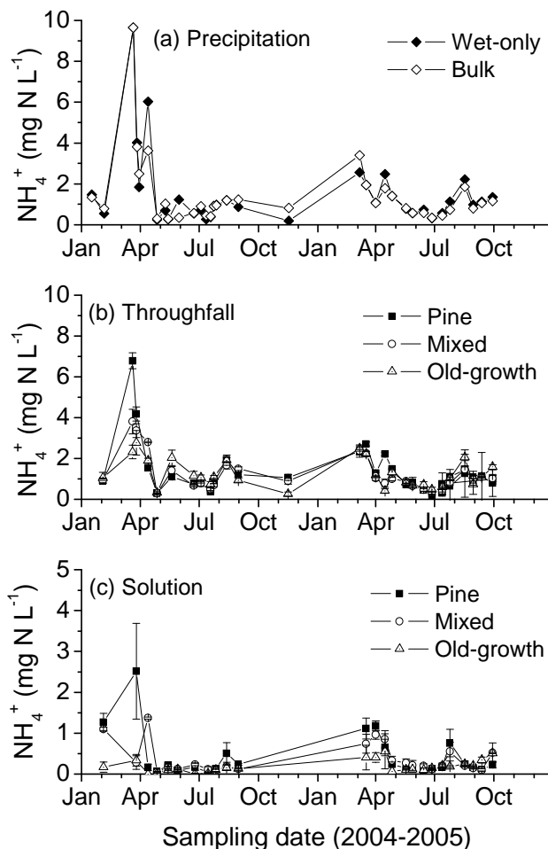
Fig. 2. \text{NH}_4^+ concentrations in precipitation (a) were measured in both wet-only collectors (automatically open during rain events) and bulk collectors (open continuously). Throughfalls (b) and soil solutions (c) were collected from Pine, Mixed, and Old-growth forests separately.
