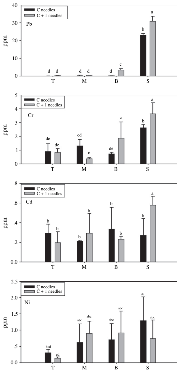
Fig. 6. Mean ± SE concentrations of Pb, Cr, Cd and Ni in different needle sections of the C and C = 1 needles of Masson pine (n = 6). The significant differences among the sections between the needles were marked in the bars with different letters according to the Paired Sample t-test. The significance is set at 0.05 level. T = tip, M = middle, B = base and S = sheath.
