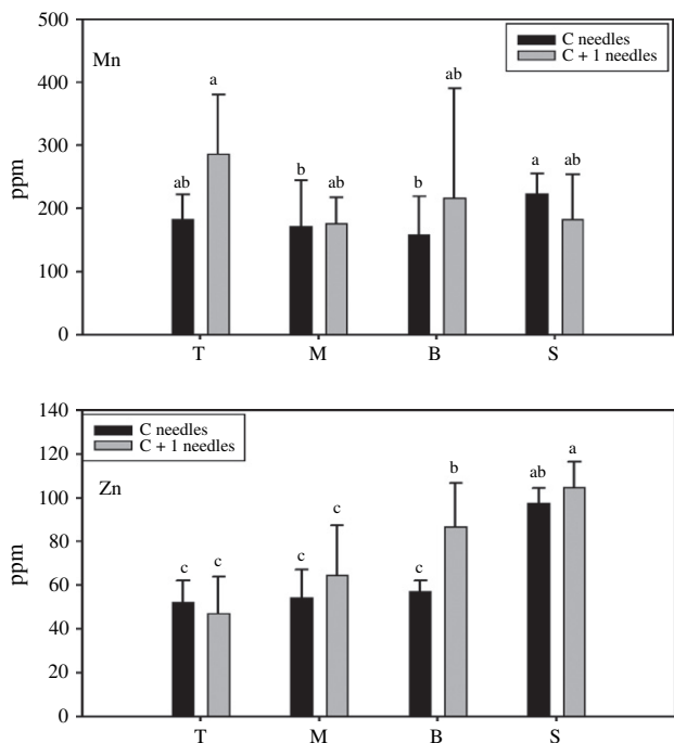
Fig. 5. Mean ± SE concentrations of Mn and Zn in different needle sections of the C and C + 1 needles of Masson pine (n = 6). The significant differences among the sections between the needles were marked in the bars with different letters according to the Paired Sample t-test. The significance is set at 0.05 level. T = tip, M = middle, B = base and S = sheath.
