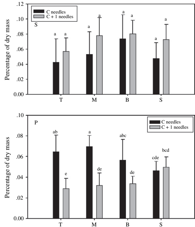
Fig. 2. Mean \pm SE contents of total S and P in different needle sections of the C and C + 1 needles of Masson pine ( n=6 ). The significant differences among the sections between the needles were marked in the bars with different letters according to the Paired Sample t -test. The significance is set at 0.05 level. T = tip, M = middle, B = base and S = sheath.
